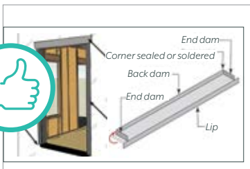
PROPERLY SEALED AND FLASHED DOORS PREVENT WATER DAMAGE Courtesy of U.S. Department of Energy
